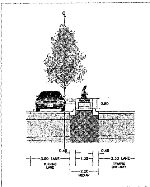
Residential Median 2.2m - A
