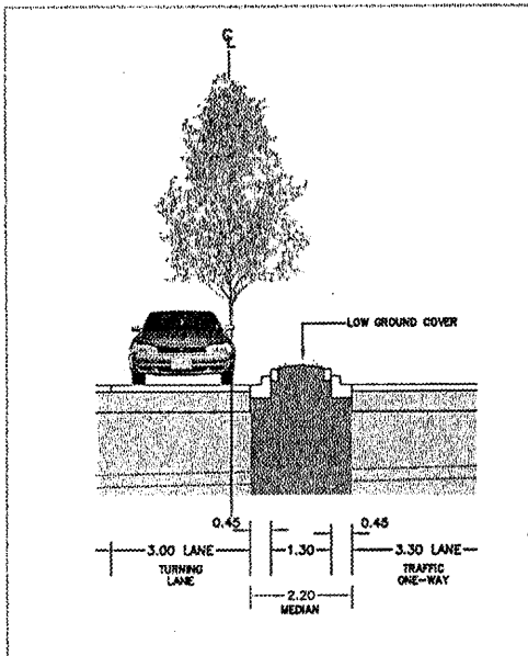
Residential Median 2.2m - B
