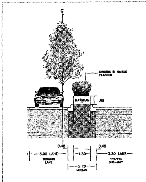
Residential Median 2.2m - C
