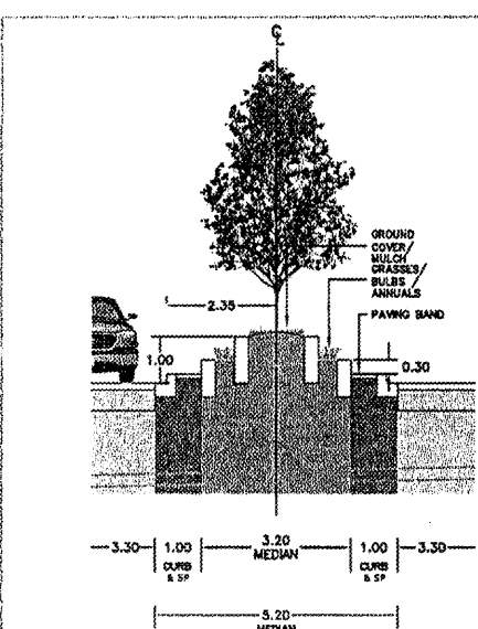
Residential Median 5.2m - C
