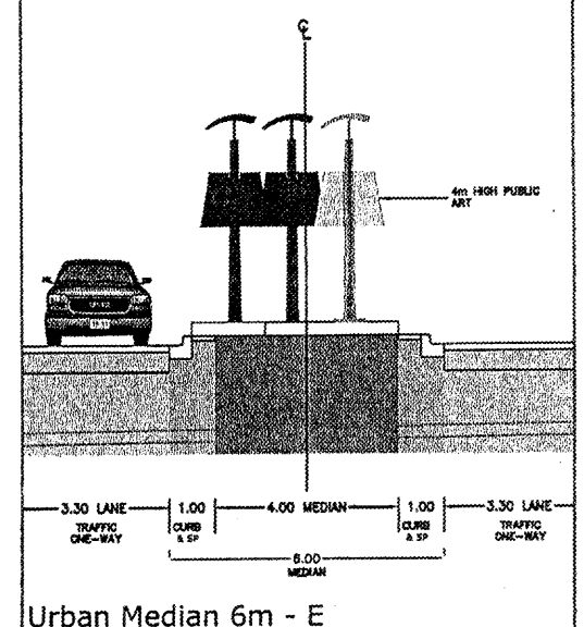
Urban Median 6m - E
