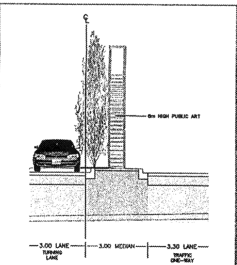
Urban Median 3m - C
