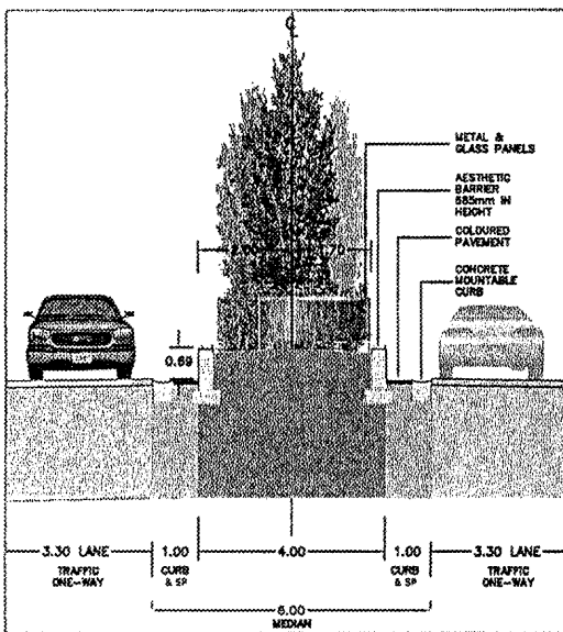
Urban Median 6m - C
