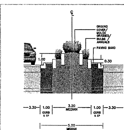
Residential Median 5.2m - C Alternate
