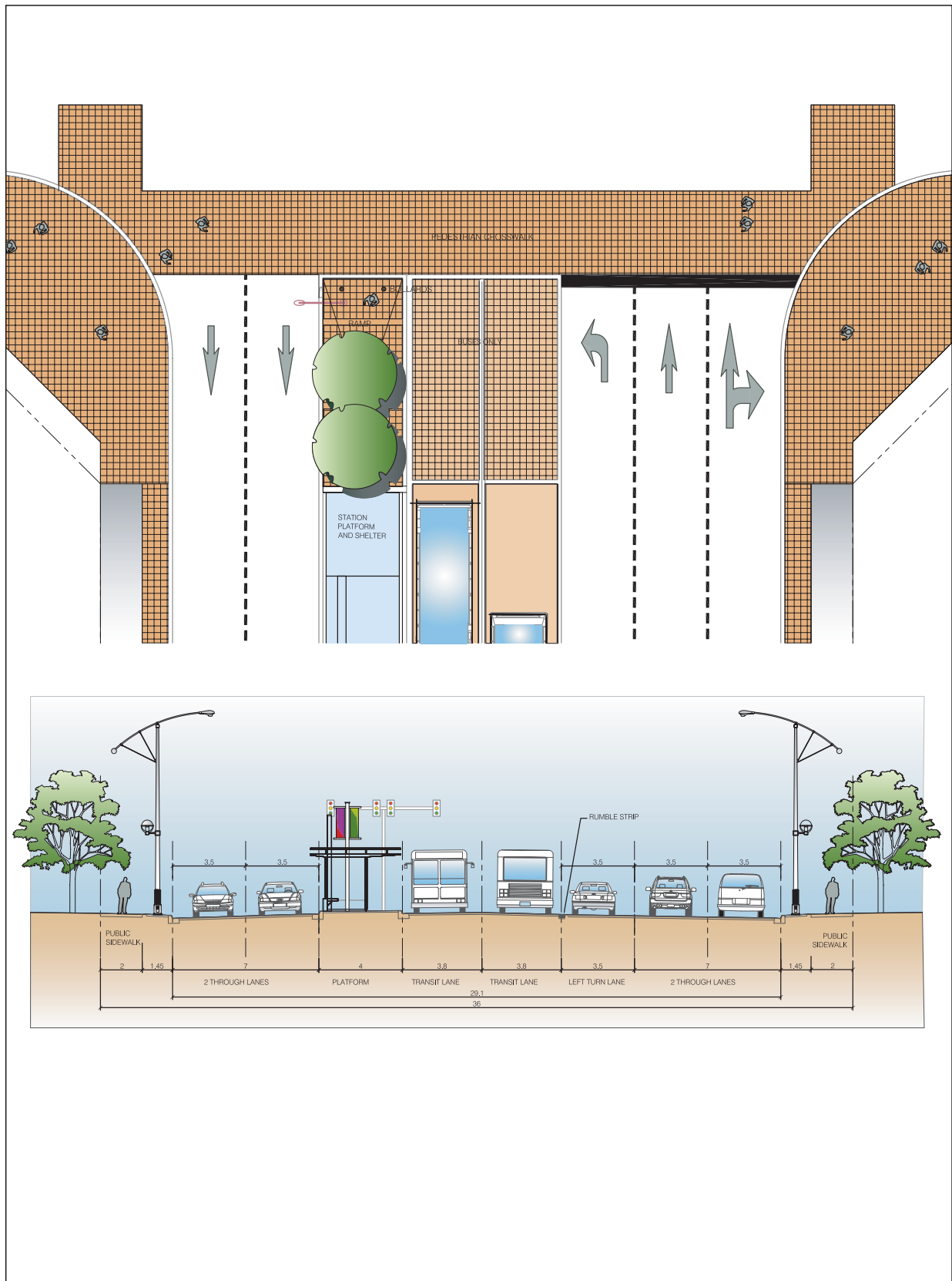
TYPICAL MEDIAN STATION CROSS-SECTION HIGHWAY 7 TRANSITWAY
