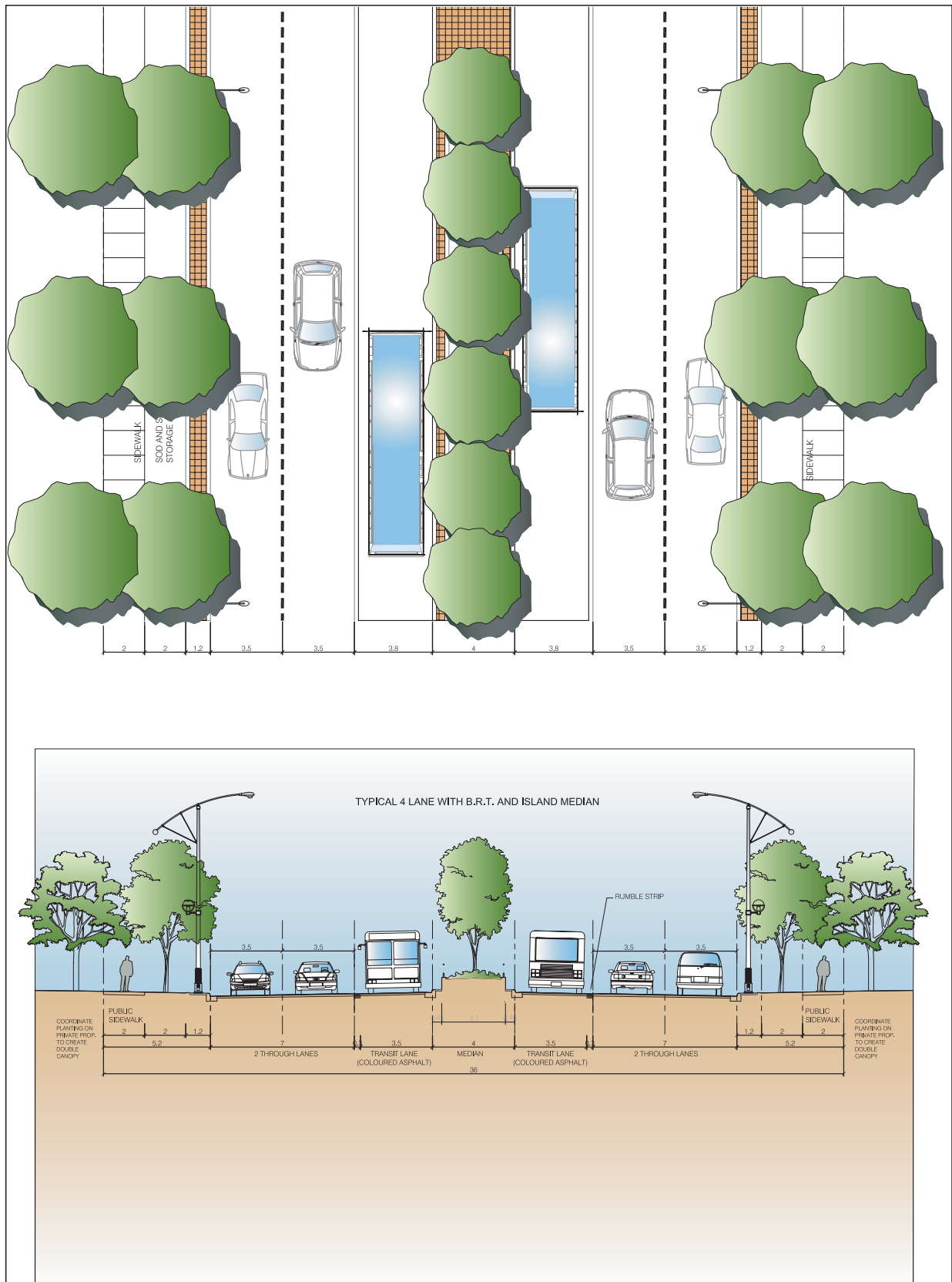
TYPICAL 36M CROSS-SECTION BETWEEN STATIONS HIGHWAY 7 TRANSITWAY
