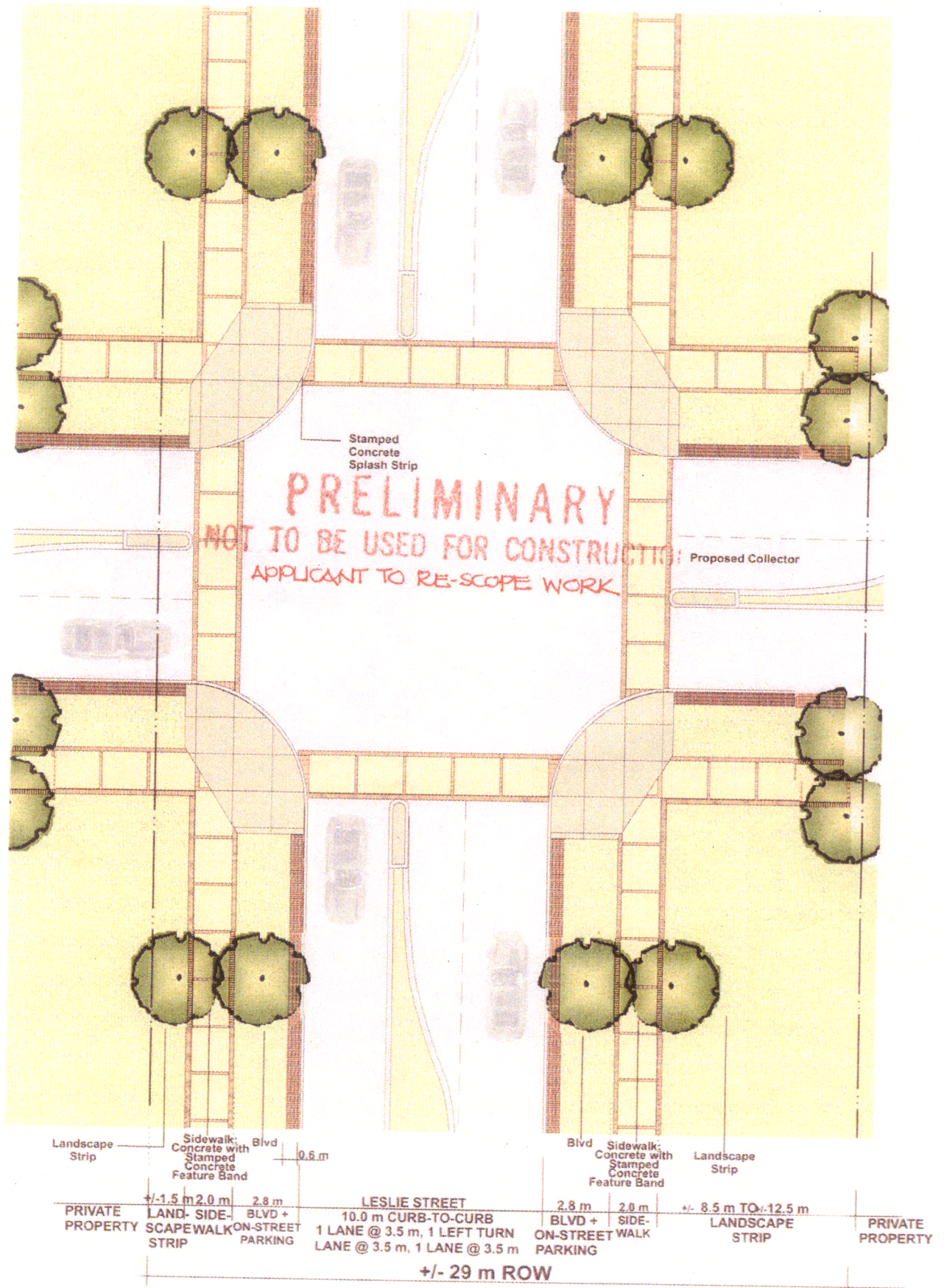
LESLIE STREET - Possible Left Turn Lane Intersection Plan at Intersections
