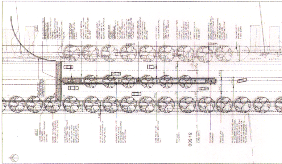
TYPICAL PLAN BOULEVARD - MEDIAN
