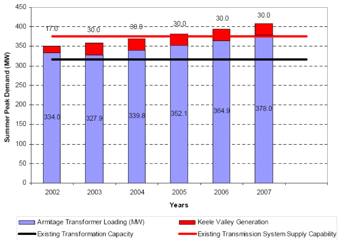
Armitage TS Peak Demand (Actual and Forecast)
