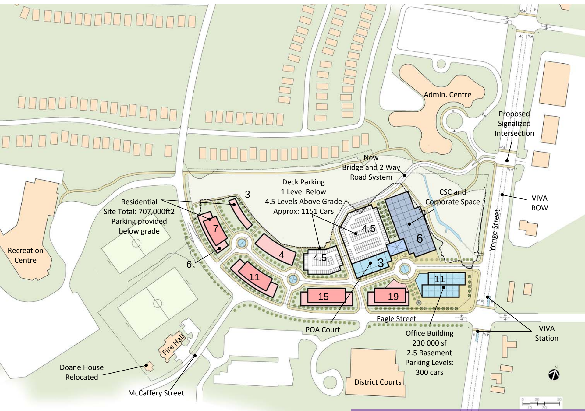
Concept Plan- Full Build Out (2.5 FSI)
