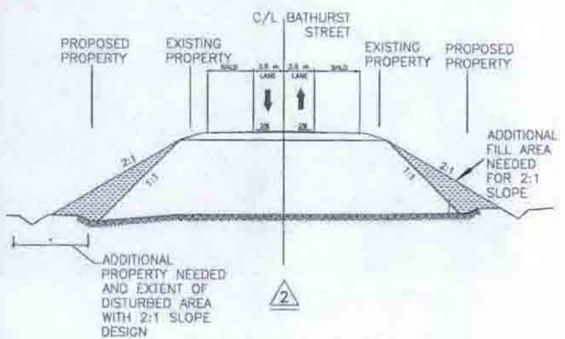
RETAINED SOIL SLOPE SECTION
