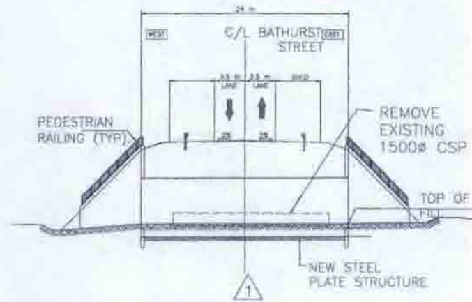
WILD LIFE CROSSING SECTION
