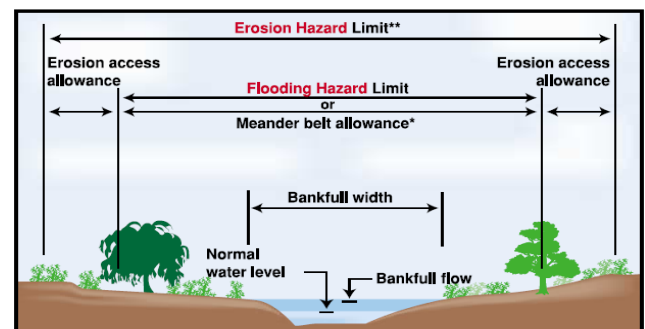
Hazard Land Cross-Section
