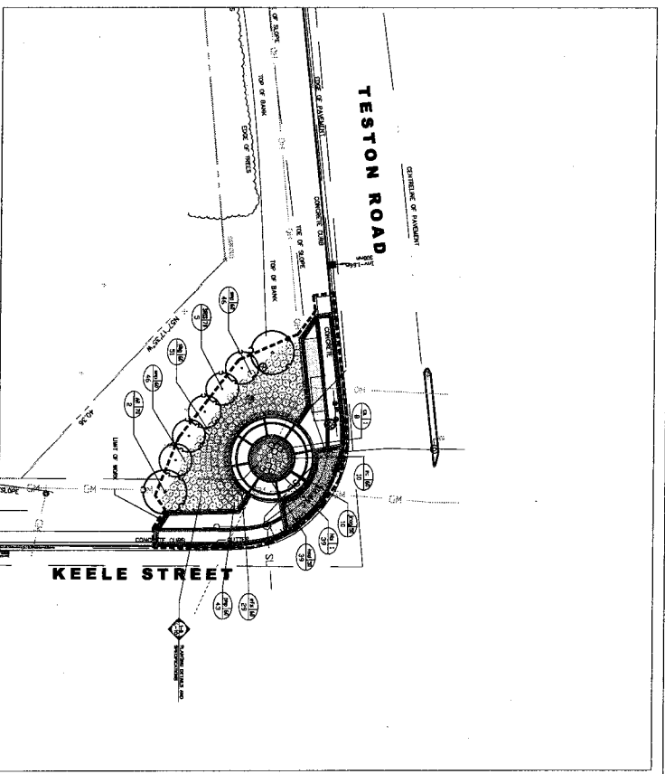
2 KEELE ST. AT TESTON RD. PLANTING PLAN 1:200
