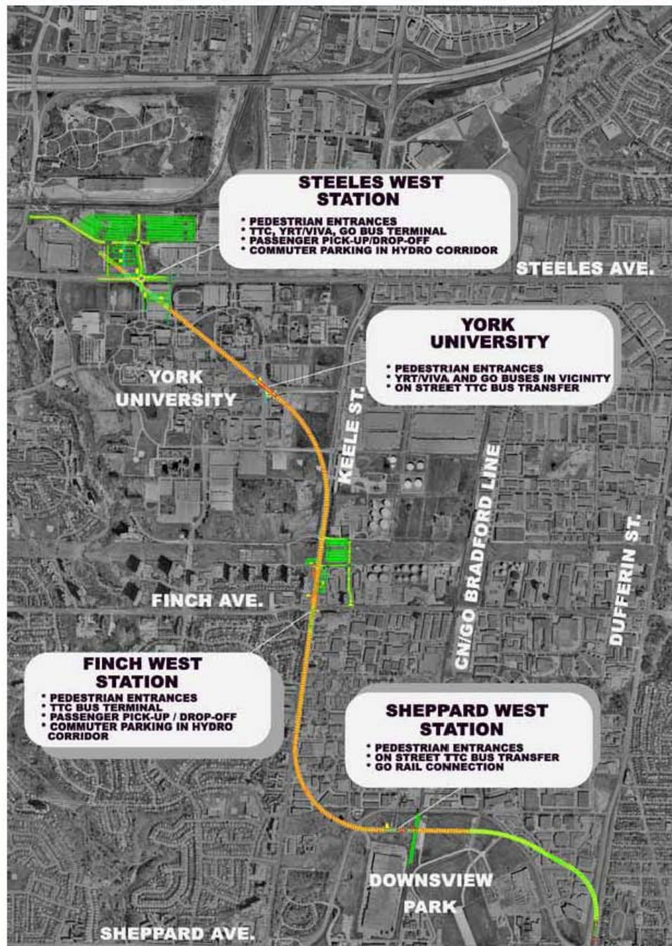
FIGURE ES – 21: RECOMMENDED SPADINA SUBWAY EXTENSION ALIGNMENT
